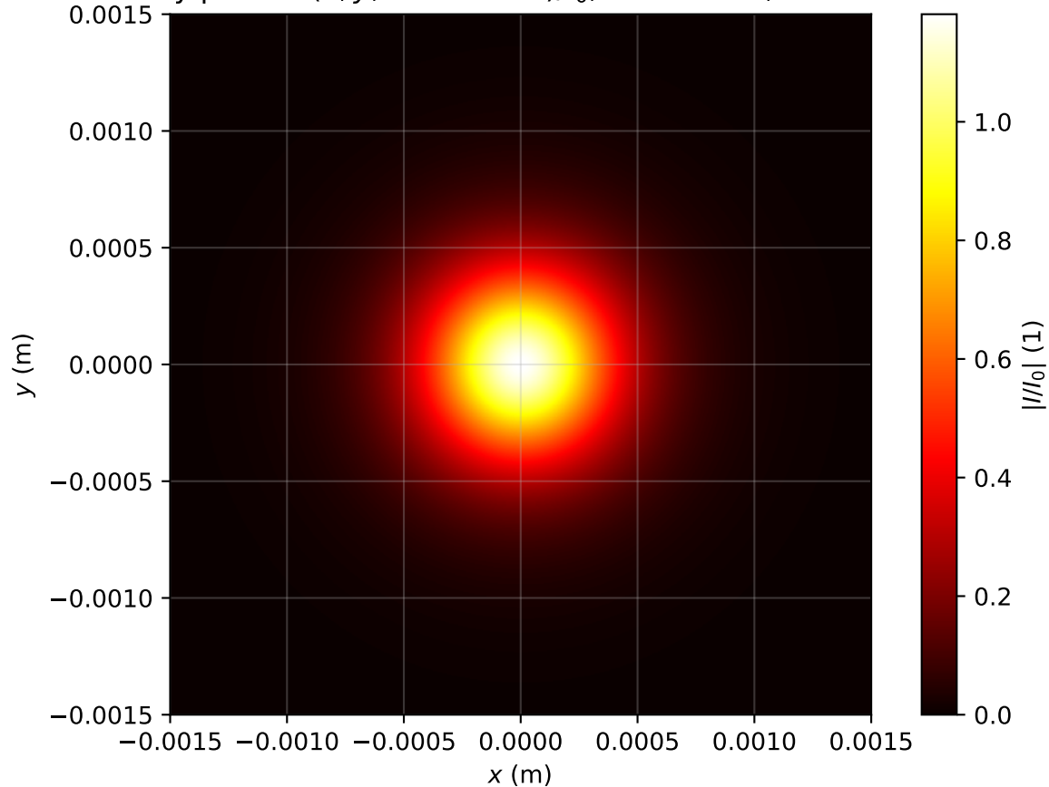
Intensity profile I(x, y, z = 1.592m)/I_0 , Pin=0.7Pcr, artificial time
